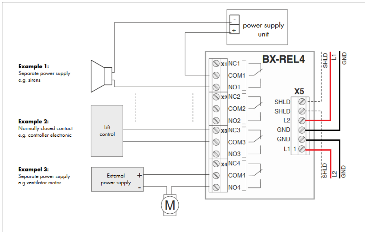
MODUL BX-REL4
